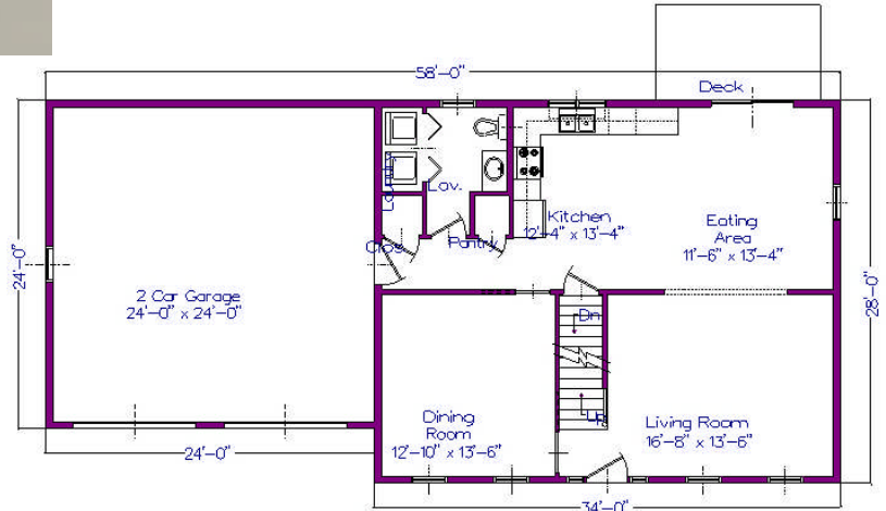
First Floor Plan Approximate Living Area: 952 s.f.
