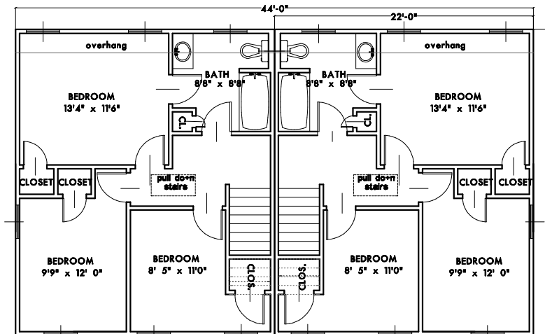
SECOND FLOOR PLAN APPROXIMATE LIVING AREA: 572 S.F.
