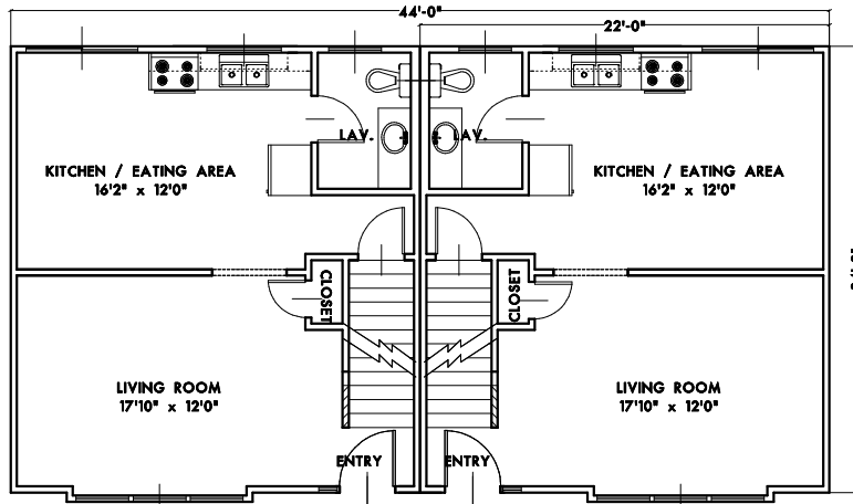
FIRST FLOOR PLAN APPROXIMATE LIVING AREA: 528 S.F.
