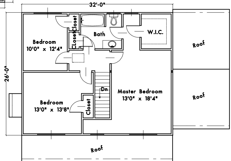
SECOND FLOOR PLAN Approximate Living Area: 832 s.f.
