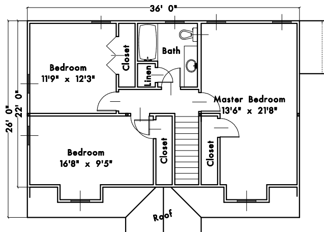
SECOND FLOOR PLAN Approximate Living Area: 816 s.f.
