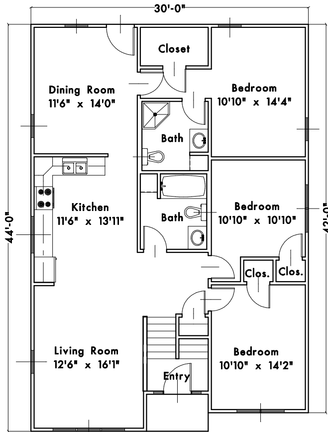
30'0" x 42'0" / 44'0" RAISED RANCH
