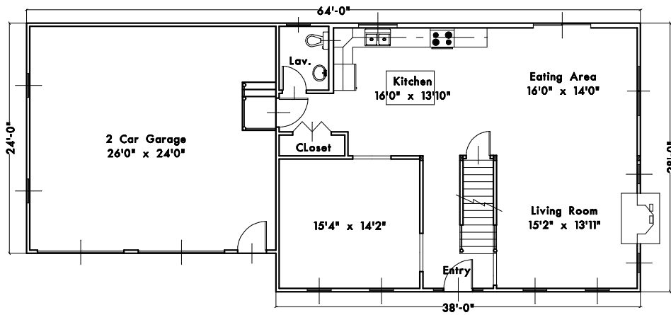
38'-0" x 28'-0" COLONIAL w/ 2 CAR GARAGE
