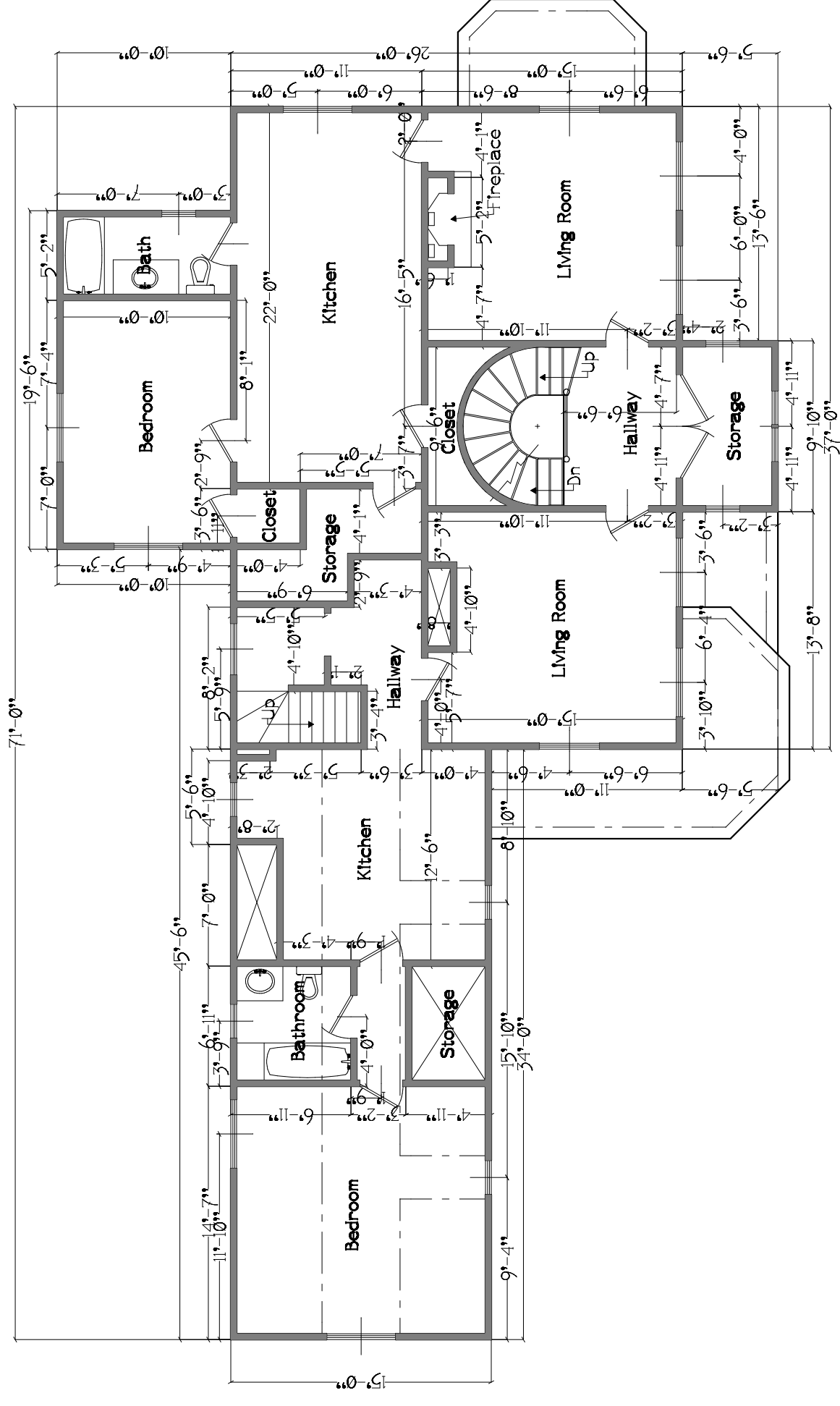
EXISTING SECOND FLOOR PLAN Approximate Living Area: 1,721 s.f.
