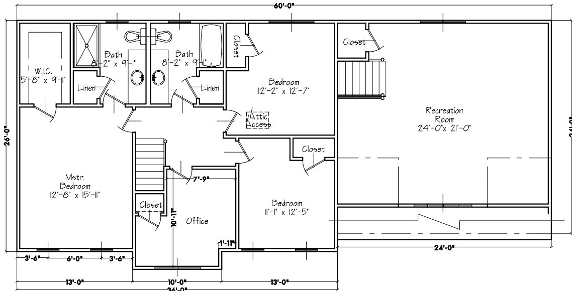
SECOND FLOOR PLAN Approximate Living Area: 1,461 s.f.
