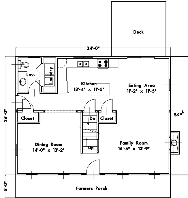
34'-0" x 26'-0" Colonial w/Farmers Porch & Garage Underneath
