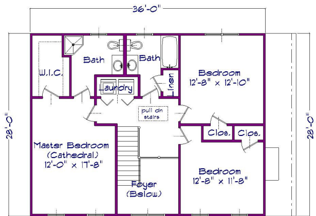
SECOND FLOOR PLAN APPROXIMATE LIVING AREA: 1,008 S.F.
