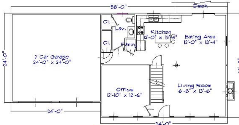
First Floor Plan Approximate Living Area: 952 S.F.
