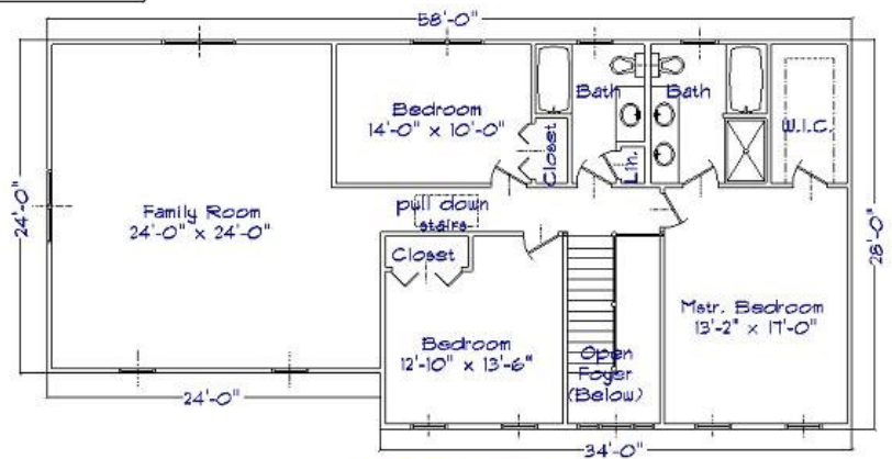
Second Floor Plan Approximate Living Area: 1,528 S.F.
