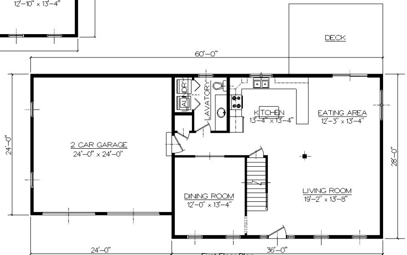
First Floor Plan Approximate Living Area: 1,008 s.f.
