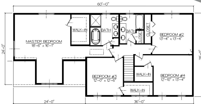
Second Floor Plan Approximate Living Area: 1,498 s.f.
