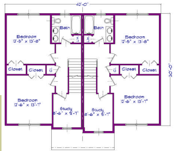
Second Floor Plan Approx. Living Area: (Each Unit): 638 s.f.
