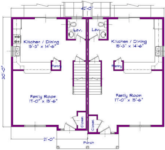
First Floor Plan Approx. Living Area: (Each Unit): 638 s.f.
