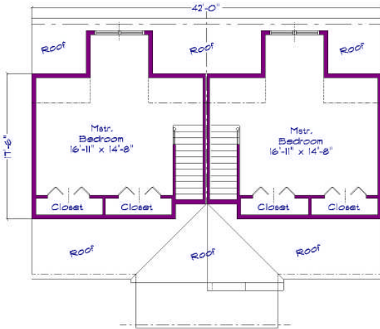
Third Floor Plan Approx. Living Area: (Each Unit): 400 s.f.
